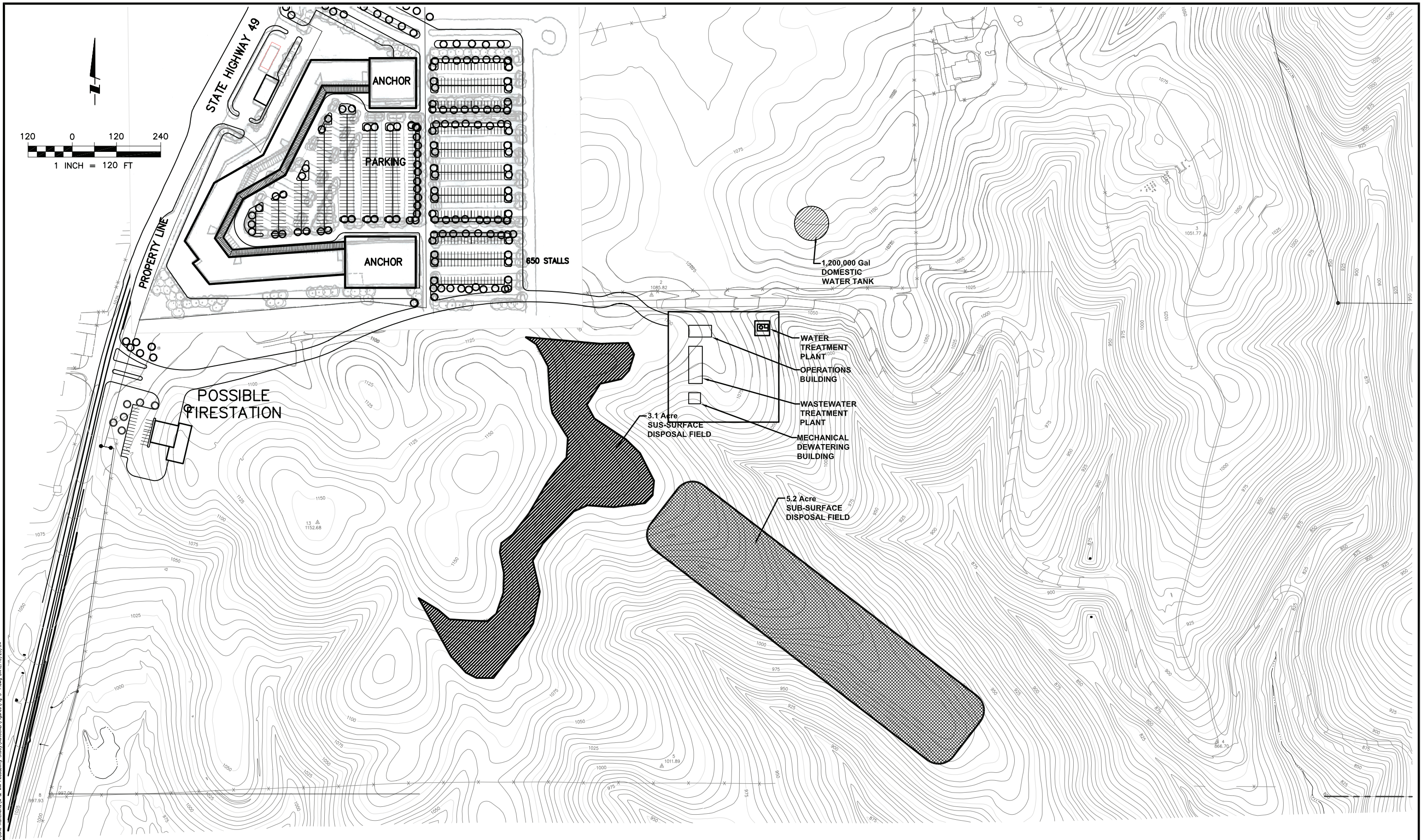
Figure 3-7 Lone Casino and Hotel Feasibility Study Water Treatment, Wastewater Treatment, and Disposal Alternative D
