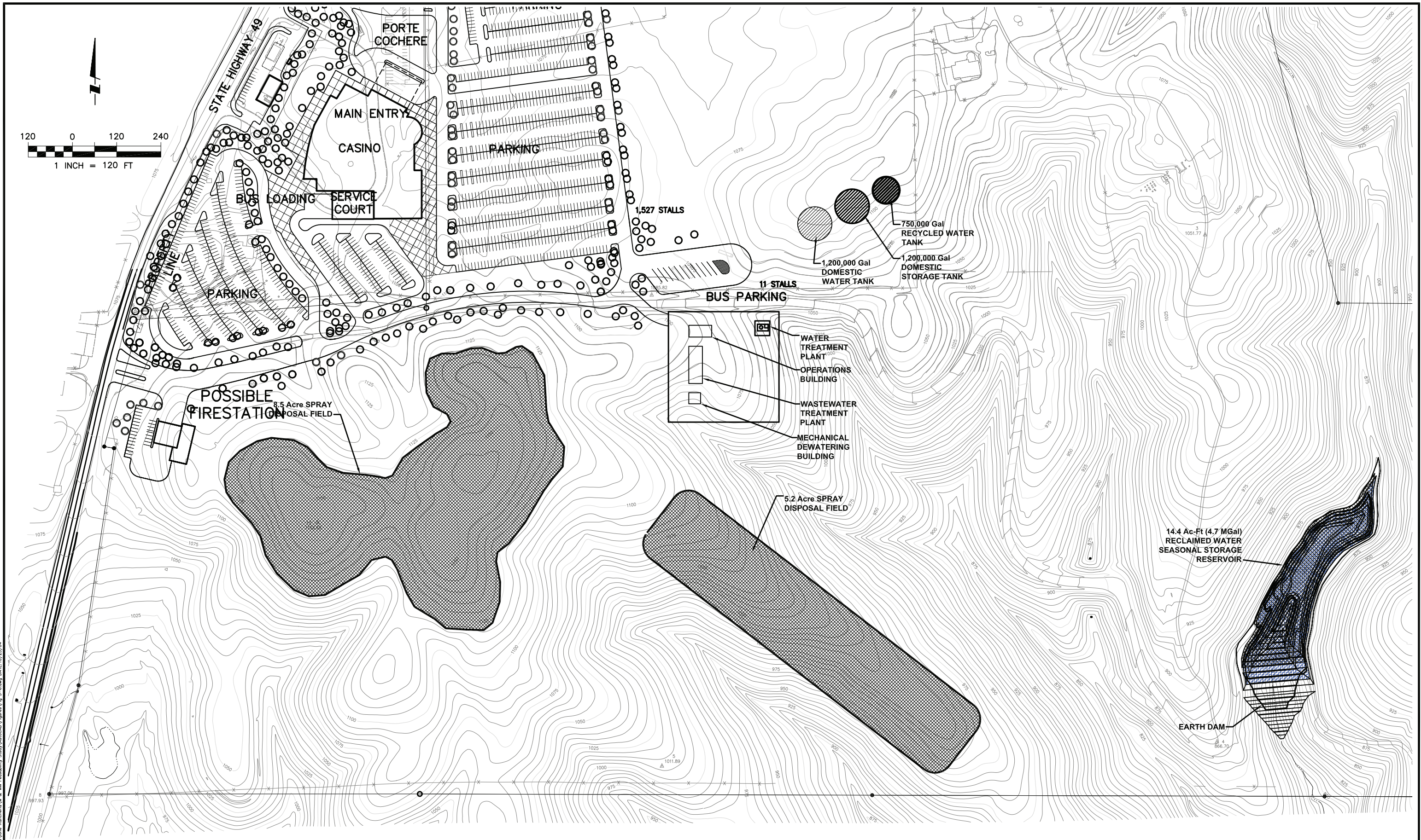
Figure 3-6 Lone Casino and Hotel Feasibility Study Water Treatment, Wastewater Treatment, and Disposal Alternative C
