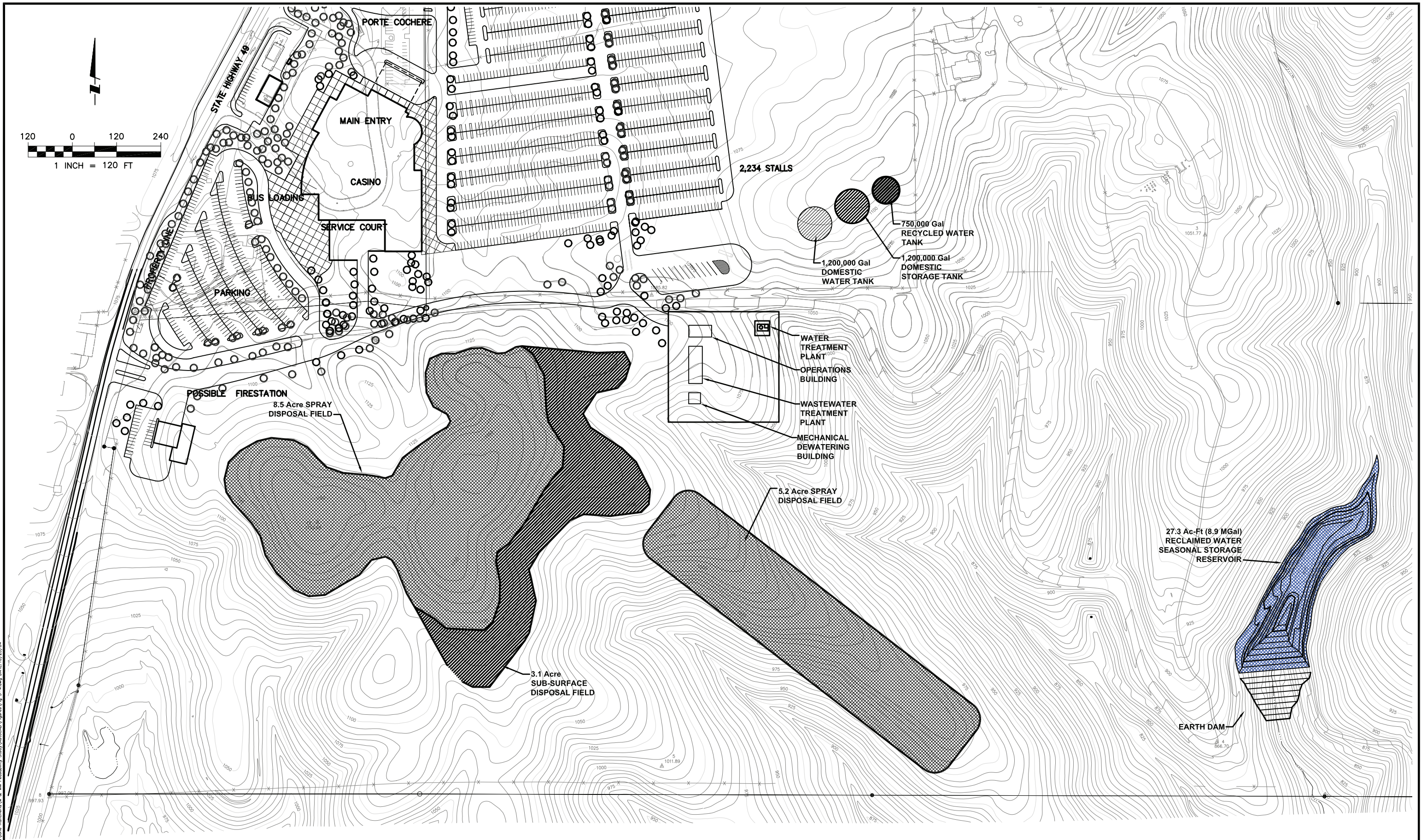
Figure 3-4 Lone Casino and Hotel Feasibility Study Water Treatment, Wastewater Treatment, and Disposal Alternative B, Phase I
