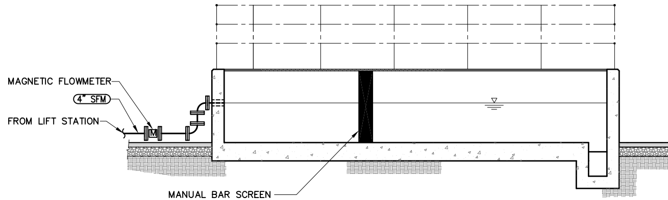
Figure 5-2 Ione Casino and Hotel Feasibility Study Typical Headworks
