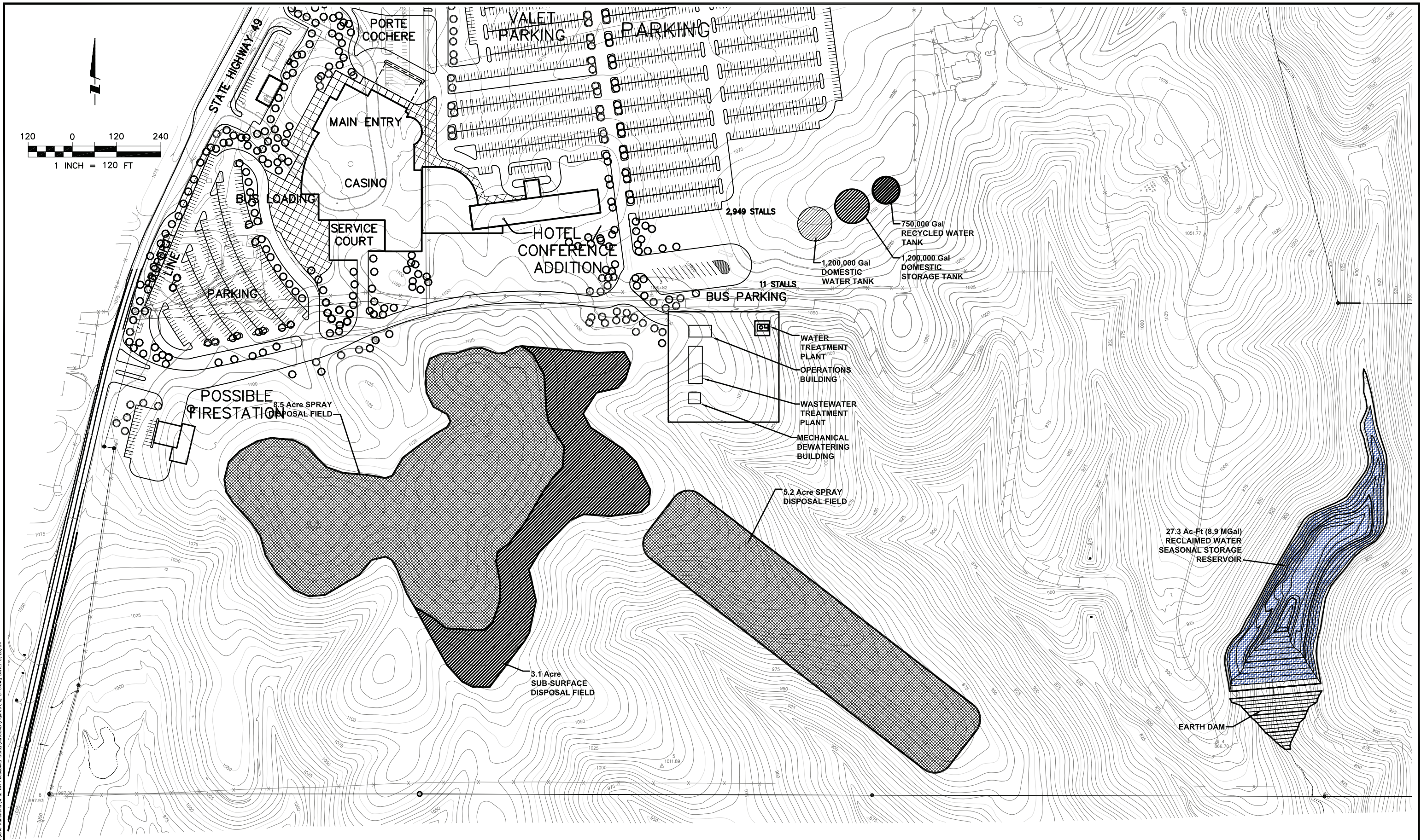
Figure 3-5 Lone Casino and Hotel Feasibility Study Water Treatment, Wastewater Treatment, and Disposal Alternative B, Phase II
