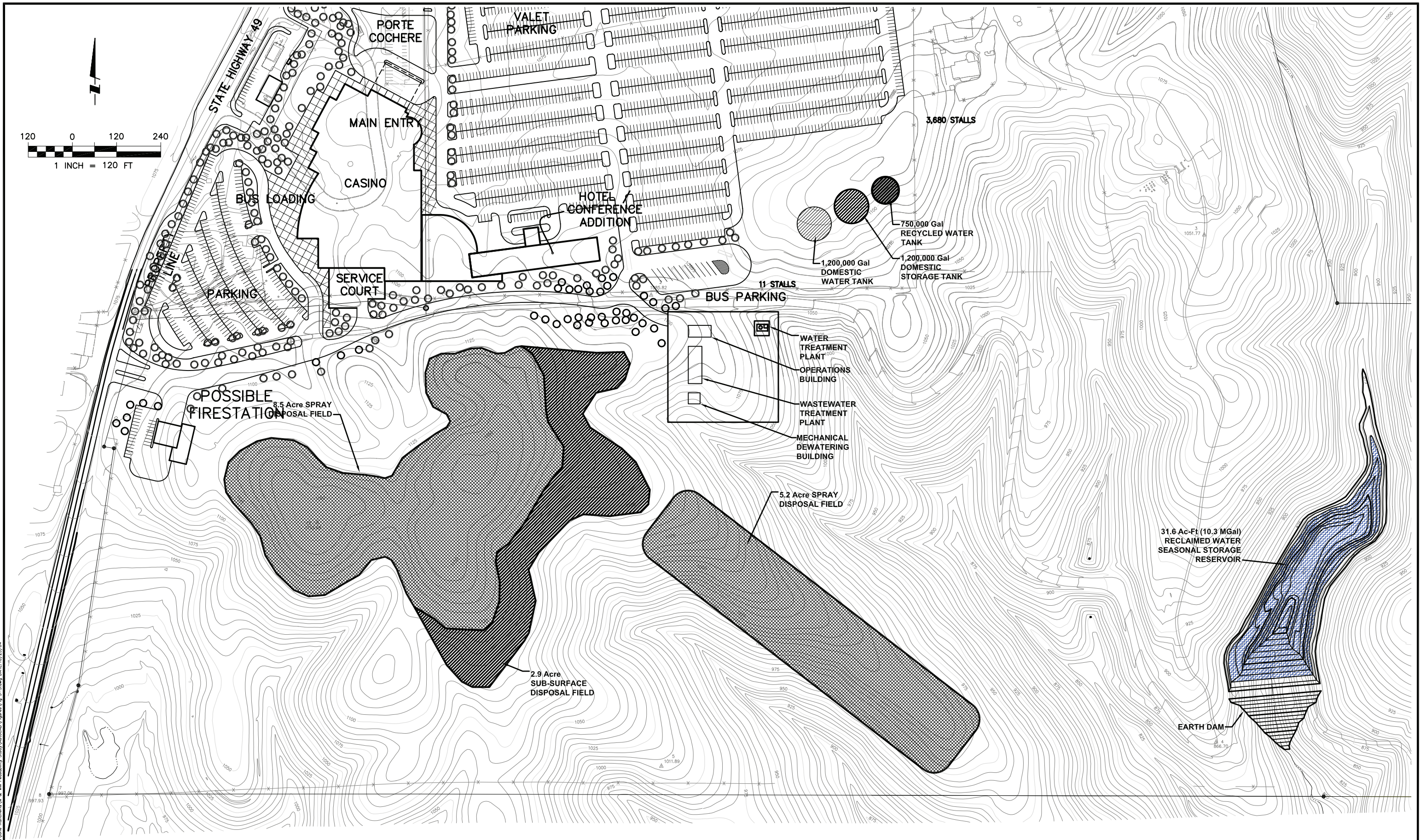
Figure 3-3 Lone Casino and Hotel Feasibility Study Water Treatment, Wastewater Treatment, and Disposal Alternative A, Phase II
